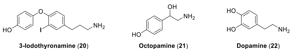
Figure 1.26 Chemical structure of 3-iodothyronamine (20) and neurotransmitters octopamine (21) and dopamine (22).
