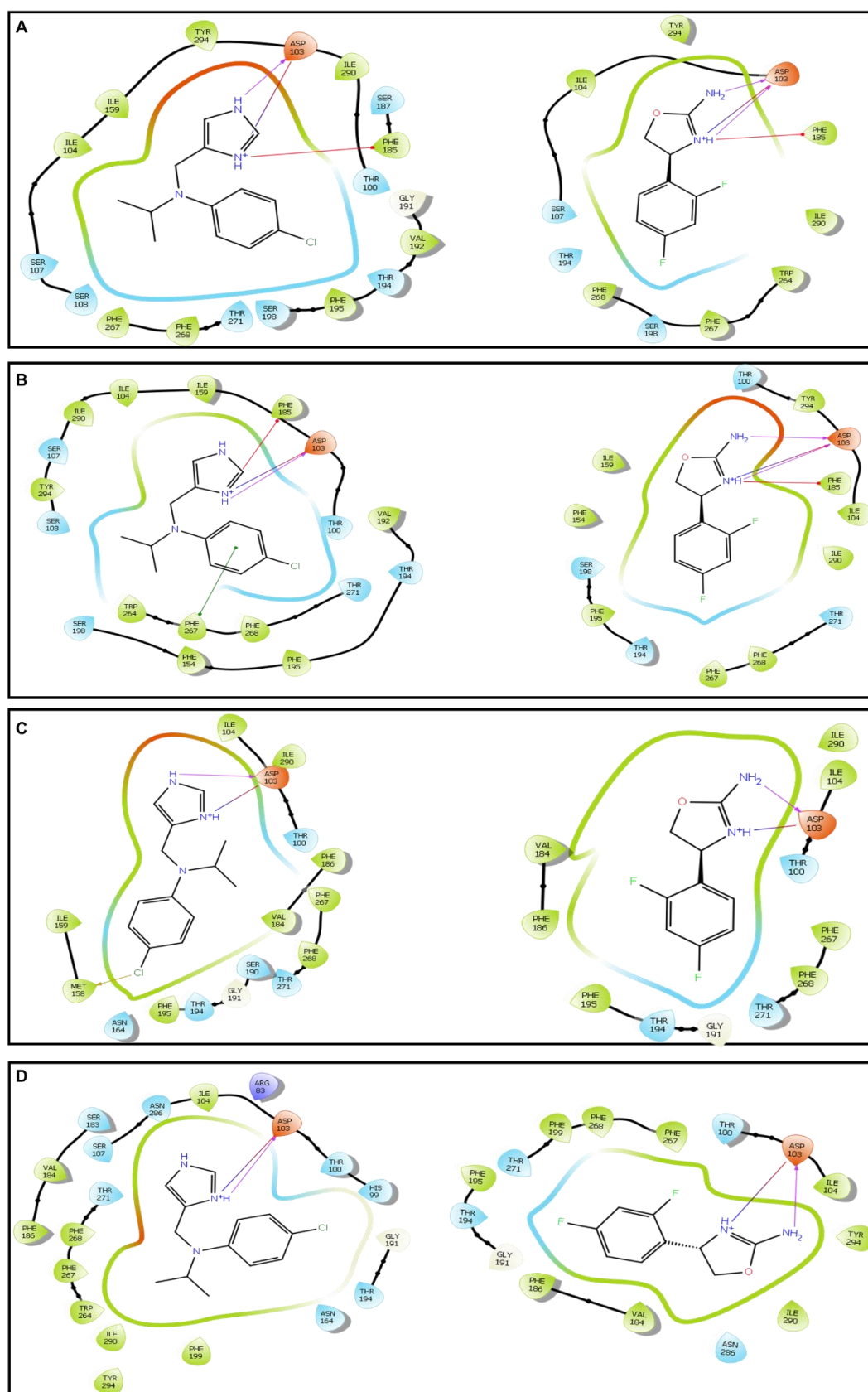
Figure 2.13 RO5073012 ( 59 , left) and ( S )-4-(2,4-difluorophenyl)-3-tritio)-4,5-dihydro-2-oxazoline ( 60 , right) interactions with hTAAR1 homology models. (A) Homology model 11. (B) Homology model 17. (C) Homology model 21. (D) Homology model 25.
