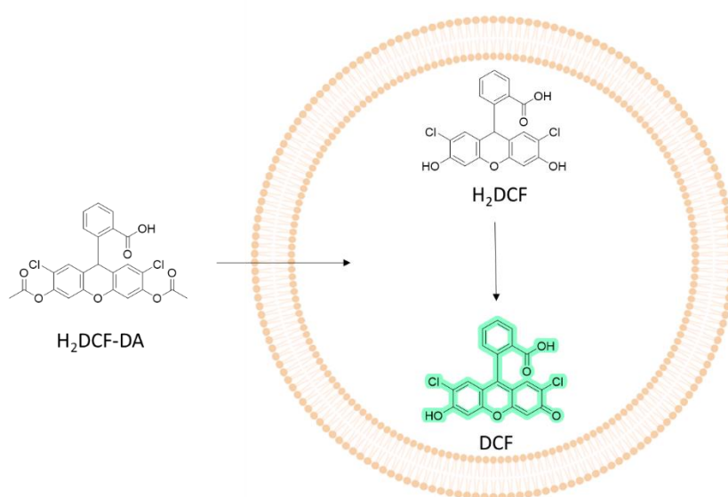
Figure 6.3 Principle of scavenging assay using 2,7-dichlorofluorescein diacetate. H_2DCF\text{-}DA enters the cell and undergoes de-esterification to form H_2DCF . The presence of reactive species causes H_2DCF to be oxidised into DCF, a highly fluorescent compound. Image created using Biorender.com.
