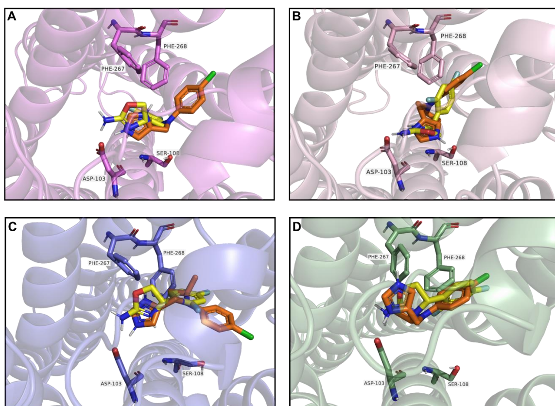
Figure 2.12 (A) Docked pose of RO5073012 ( 59 , orange) and ( S )-4-(2,4-difluorophenyl-3-tritio)-4,5-dihydro-2-oxazamine ( 60 , yellow) into homology model 11. (B) Docked pose of 59 (orange) and 60 (yellow) into homology model 17. (C) Docked pose of 59 (orange) and 60 (yellow) into homology model 21. (D) Docked pose of 59 (orange) and 60 (yellow) into homology model 25. All Images visualised down transmembrane 3. Docking performed using Schrödinger's Maestro and Glide 12.6 packages and images created using PyMOL 4.6.0.
