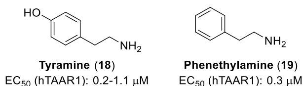
Figure 1.24 Chemical structure of tyramine ( 18 ) and phenethylamine ( 19 ).
