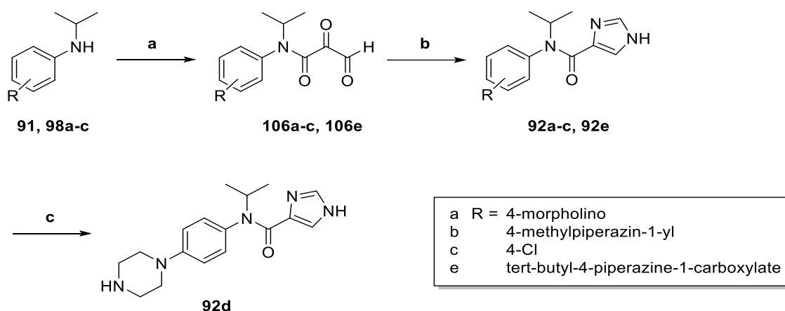
Scheme 5.8 Proposed synthesis of analogues 92a-d .
