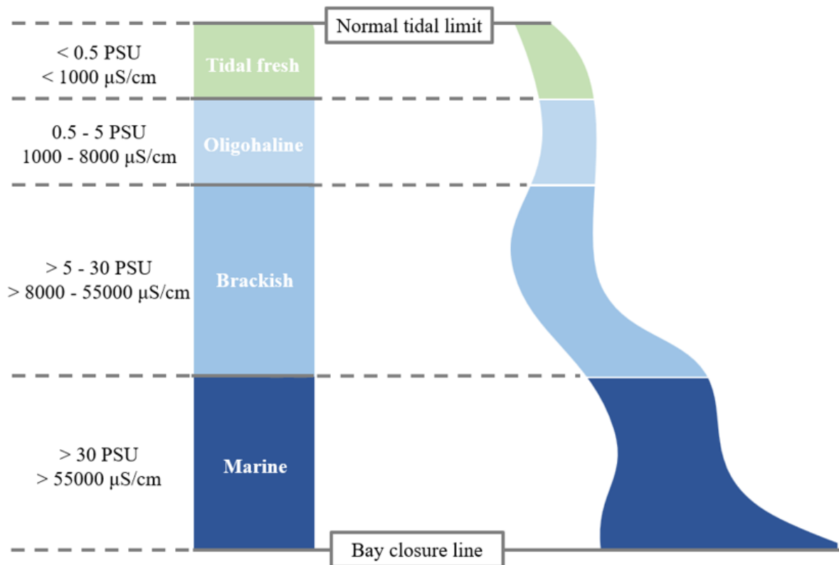
Figure 1. Salinity and conductivity boundaries used to define each estuarine zone. Tidal waters in mainland England and Wales were classified as ‘tidal freshwater’ (< 0.5 PSU or 1000 \mu\text{S/cm} ), ‘oligohaline’ (0.5-5 PSU or 1000-8000 \mu\text{S/cm} ), ‘brackish’ (5-30 PSU or 8000-55000 \mu\text{S/cm} ), or ‘marine’ (> 30 PSU or 55000 \mu\text{S/cm} ).
