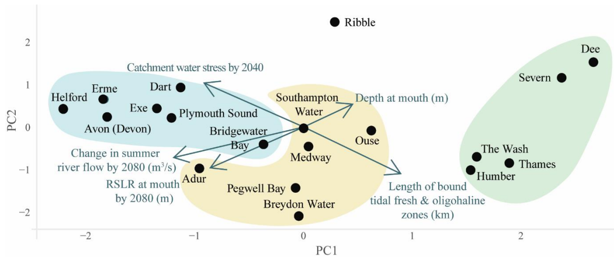
Figure 6. Principal component analysis (PCA) depicting the relationship between the bound estuaries containing oligohaline and/or tidal freshwater zones and the vulnerability data (shown in Supplementary Data Table 4). Clusters are shaded to aid interpretation. The blue cluster are ria or bar-built estuaries in the south west of England, the green cluster consists of coastal plain and embayment estuaries with deep mouths and large tidal freshwater and/or oligohaline extents and the yellow cluster coastal plain, bar built and embayment estuaries in the south and south east England.
