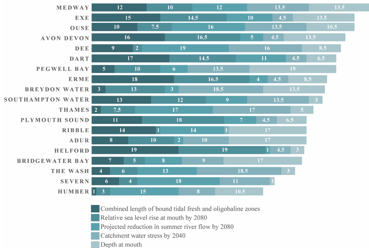
Figure 4 Ranking of 19 UK estuaries on their vulnerability to estuarine squeeze. Each estuary was assigned a rank (or tied rank, where applicable) for the following indices; combined length of tidal freshwater and oligohaline zones; relative projected sea level rise at the estuary mouth, predicted future river flow, catchment water stress, and depth at mouth
