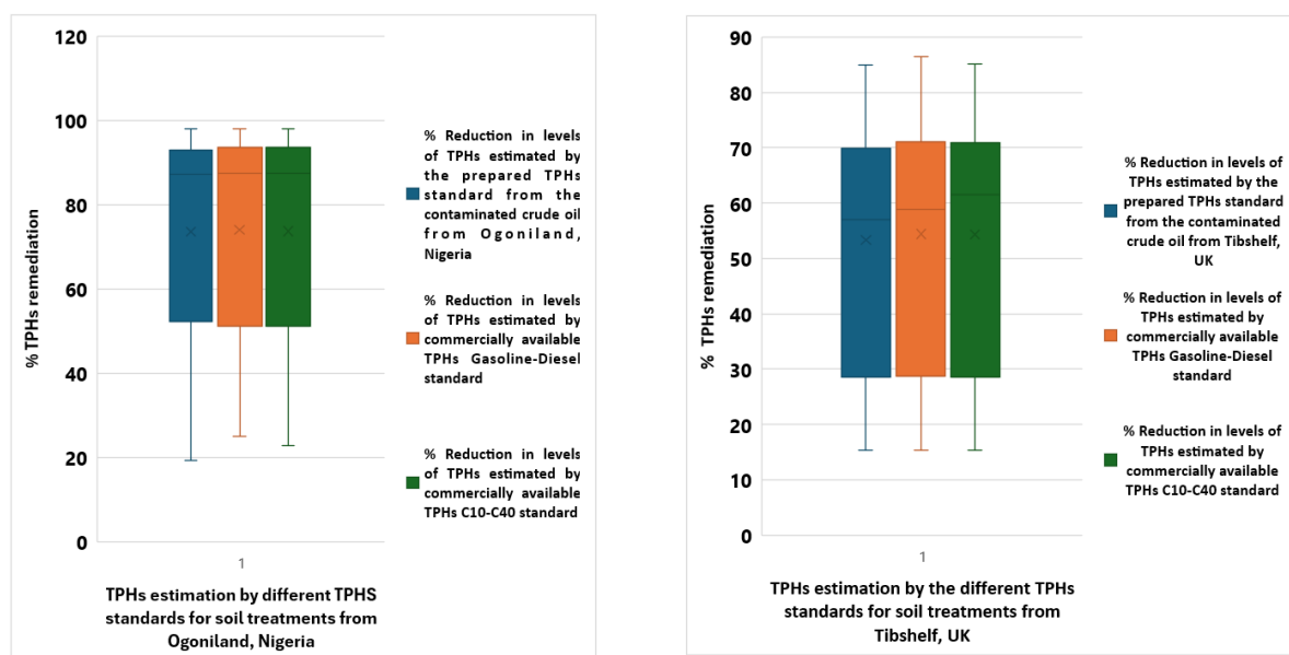
Figure 2. Box and Whisker plots for % reduction in TPHs levels in the different soil treatment for Ogoniland, Nigeria; and Tibshelf, Derbyshire, UK, using the different TPHs standards.
